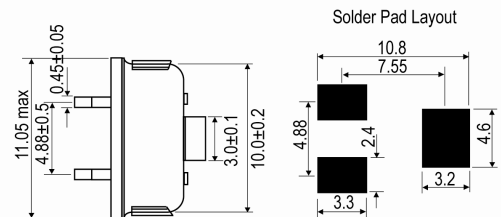
Outline (mm) -Gull-Wing = Gull-Wing
